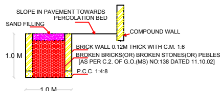
SECTION OF RAIN WATER PERCOLATION BED
