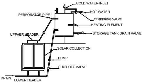
DETAILS OF SOLAR WATER HARVESTING (NTS)
