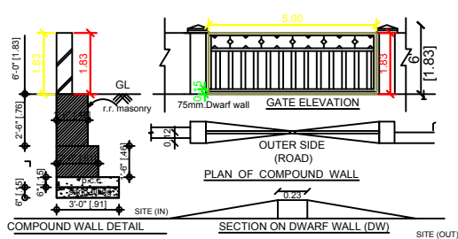
DETAILS OF COMPOUND WALL
