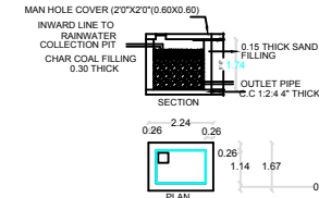
DETAILS OF RAINWATER HARVESTING
