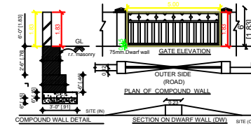
DETAILS OF COMPOUND WALL
