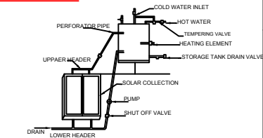
DETAILS OF SOLAR WATER HARVESTING (NTS)
