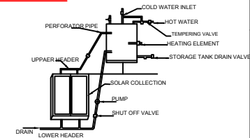
DETAILS OF SOLAR WATER HARVESTING (NTS)
