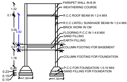
SECTION ON-AA
