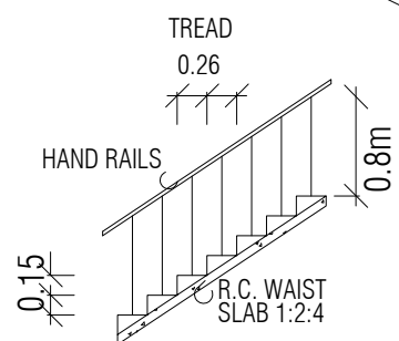
STAIRCASE DETAILS
