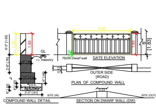
DETAILS OF COMPOUND WALL
