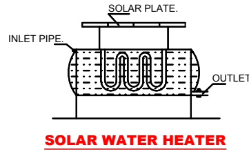
SOLAR WATER HEATER
