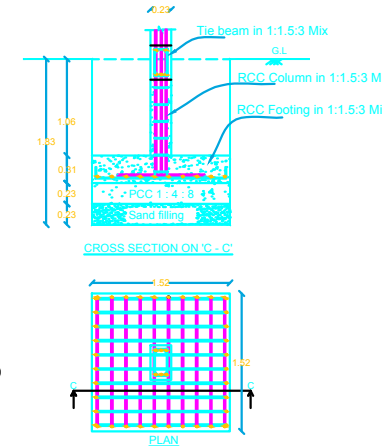
COLOUMN FOUNDATION DETAILS
