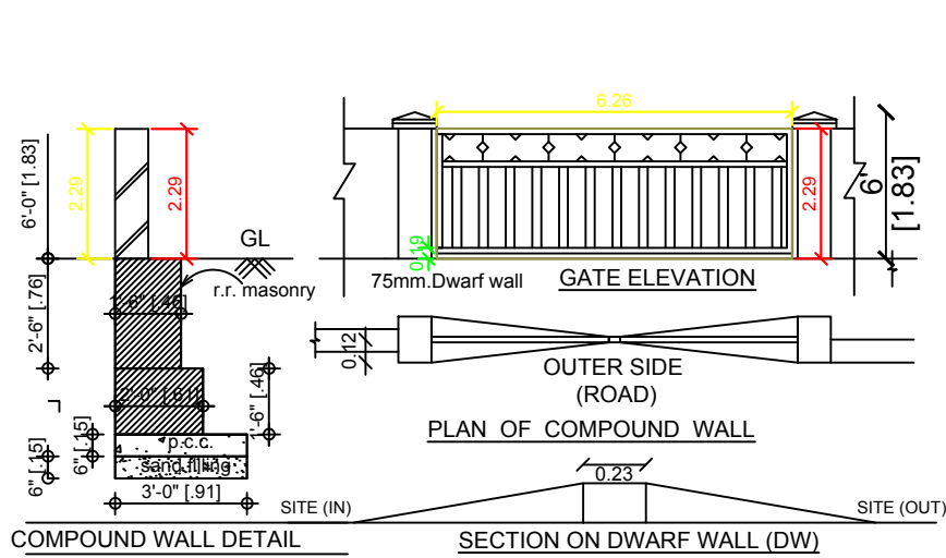
DETAILS OF COMPOUND WALL
