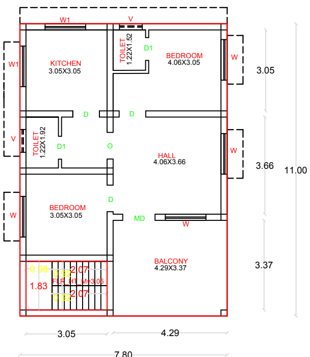
EX. FIRST FLOOR PLAN
