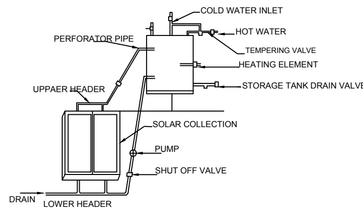
DETAILS OF SOLAR WATER HARVESTING (NTS)
