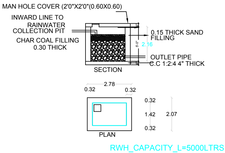
DETAILS OF RAINWATER HARVESTING
