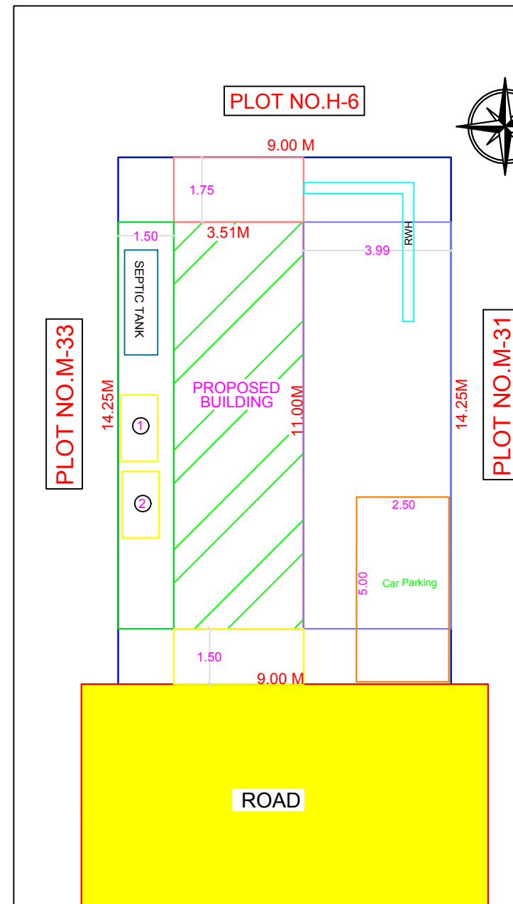
SITE PLAN
