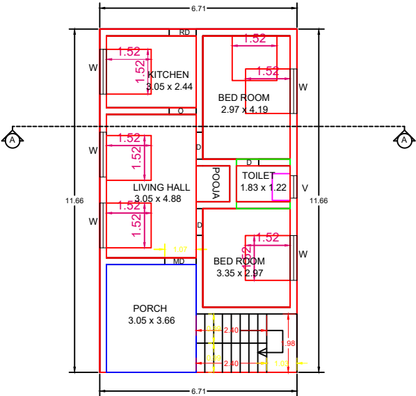
PRO.GOUND FLOOR PLAN
