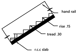
STAIR
