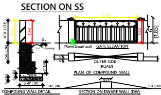
SECTION ON SS
