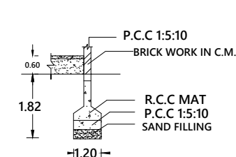
FOUNDATION DETAILS
