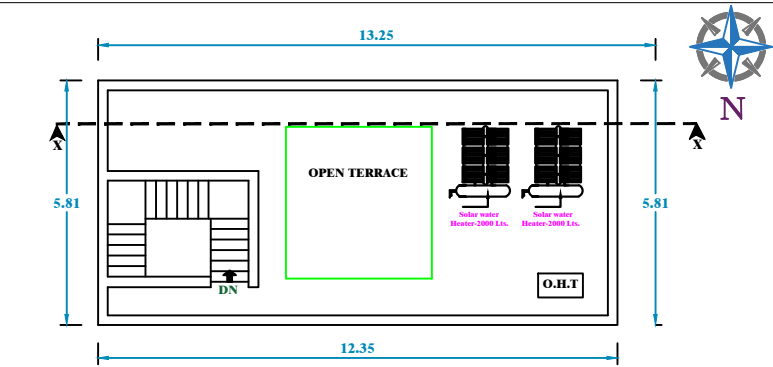
PROPOSED TERRACE FLOOR PLAN
