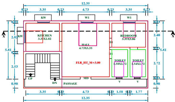
PROPOSED TYPICAL 1ST & 2ND FLOOR PLAN
