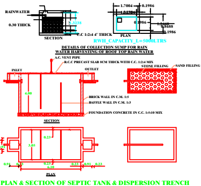
PLAN & SECTION OF SEPTIC TANK & DISPERSION TRENCH
