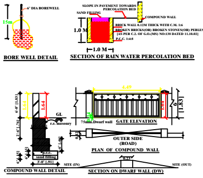
BORE WELL DETAIL
