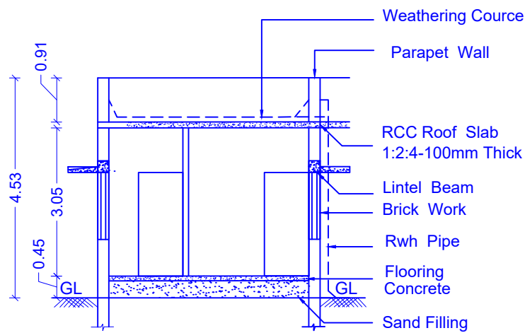
SECTION X-Y
