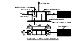
SEPTIC TANK AND TRENCH
