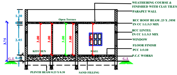
SECTION ON 'X - X'
