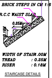
STAIRCASE DETAILS
