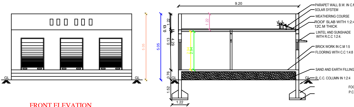
FRONT ELEVATION (SOUTH FACING)
