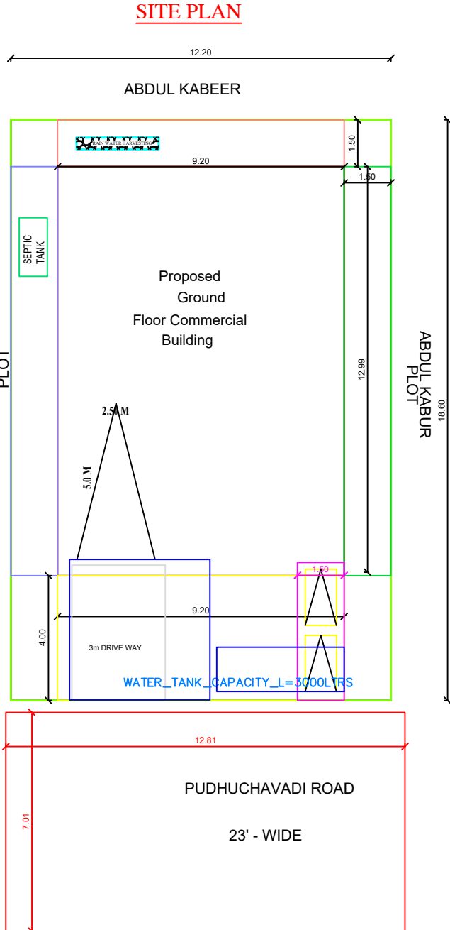
SITE PLAN
