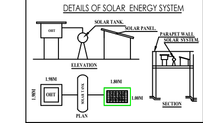
DETAILS OF SOLAR ENERGY SYSTEM
