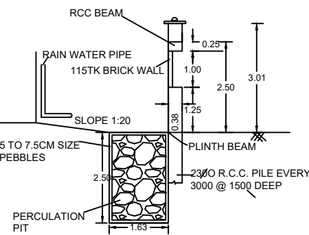
RAINWATER HARVESTING
