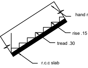
STAIR
