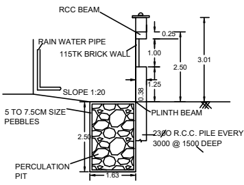
RAINWATER HARVESTING
