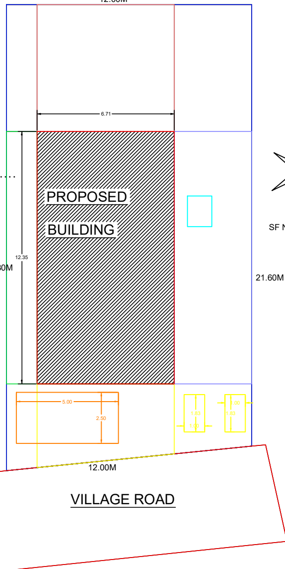
SF NO.248/16 SITE PLAN 1:100 SCALE
