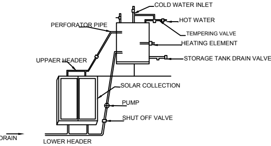
DETAILS OF SOLAR WATER HARVESTING (NTS)
