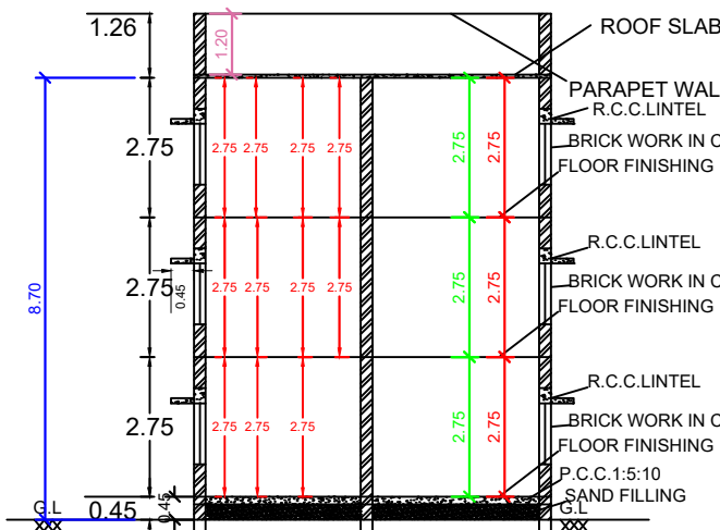
SECTION ON SS
