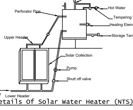
Details of solar water heater (NTS)
