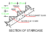
SECTION OF STAIRCASE
