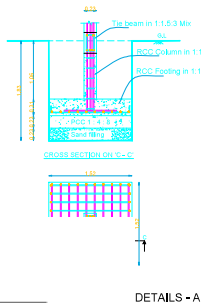
DETAILS - A
