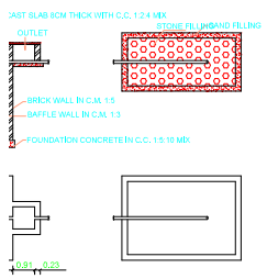
TANK & DISPERSION TRENCH
