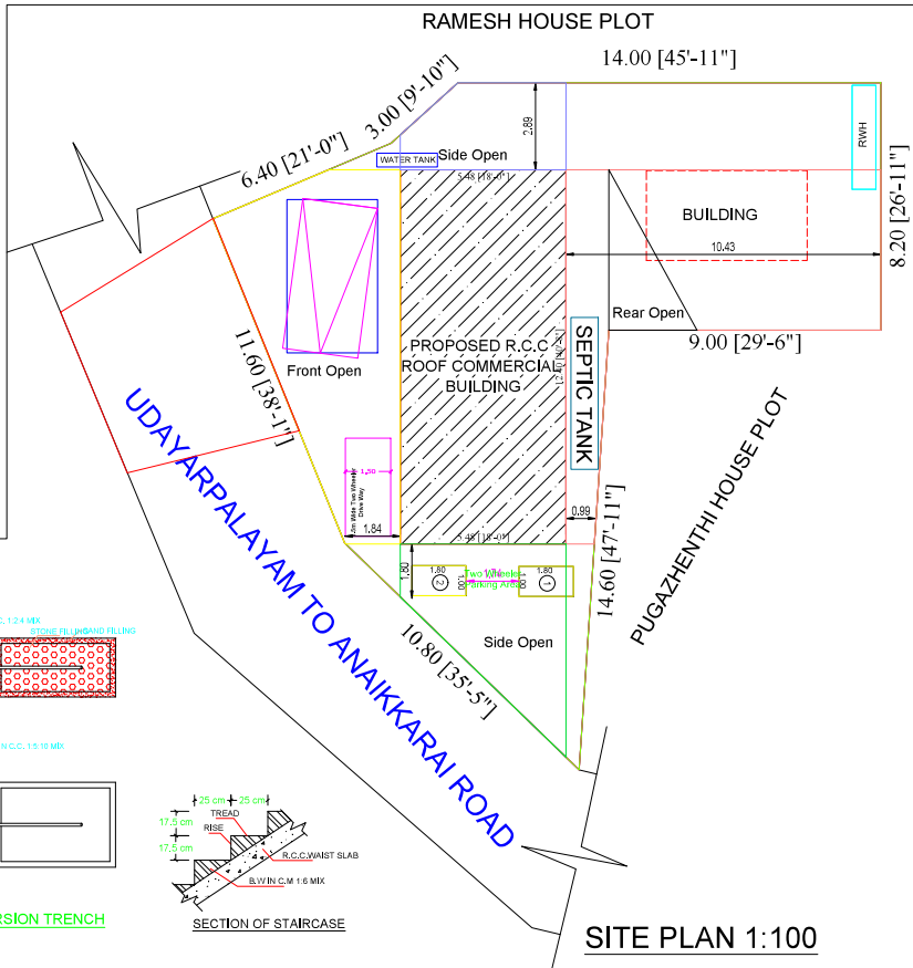
DETAILS - A
