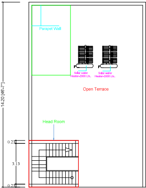
POSED) HEAD ROOM & TERRACE PLAN
