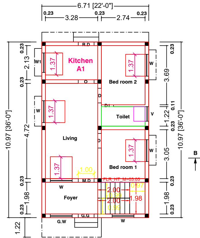
FLOOR-0 (GROUND) PLAN ( FACING NORTH )
