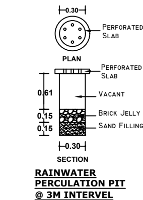
RAINWATER PERCOLATION PIT @ 3M INTERVAL
