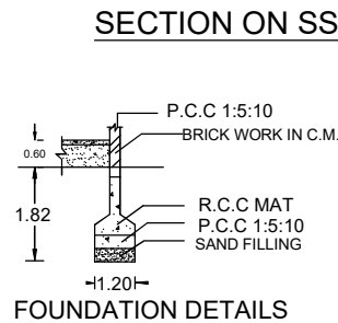
FOUNDATION DETAILS
