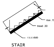
STAIR
