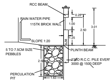
RAINWATER HARVESTING
