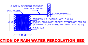
SECTION OF RAIN WATER PERCOLATION BED
