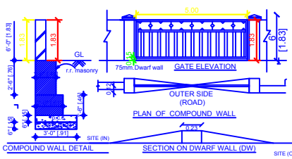
DETAILS OF COMPOUND WALL
