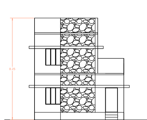
FRONT ELEVATION
