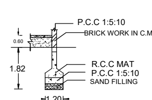
FOUNDATION DETAILS
