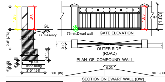
SECTION ON DWARF WALL (DW)
