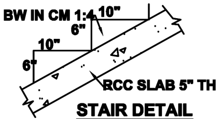
STAIR DETAIL
