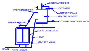
DETAILS OF SOLAR WATER HARVESTING (NTS)
