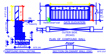
DETAILS OF COMPOUND WALL
