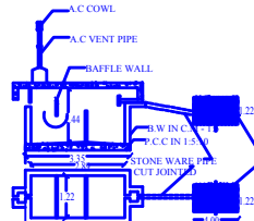
SEPTIC TANK DETAILS
