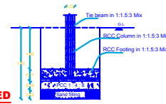
BORE WELL DETAIL
