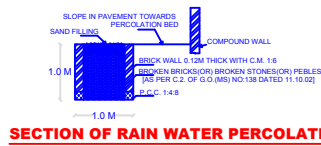
SECTION OF RAIN WATER PERCOLATION BED
