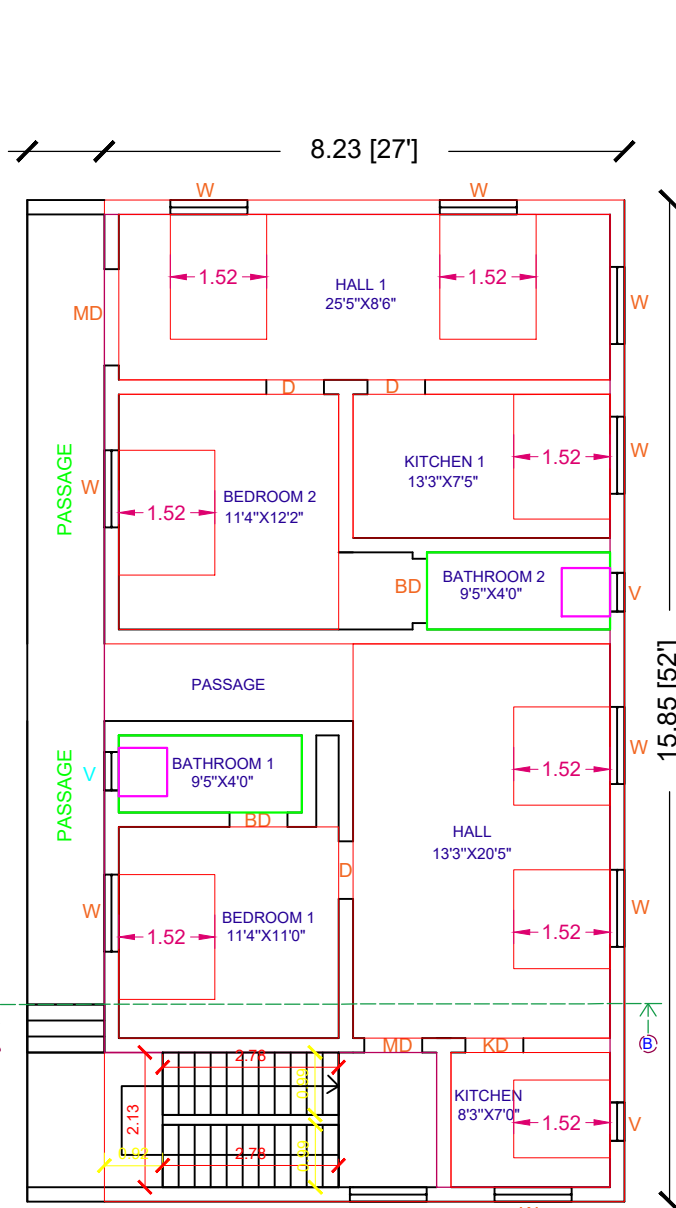
PROPOSED FIRST FLOOR
