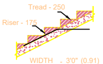
STAIR-CASE DETAILS (NOT TO SCALE)
