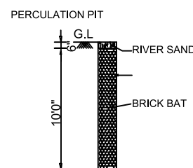
PERCOLATION PIT
