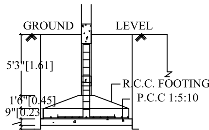
FOUNDATION DETAILS
