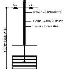
BORE WELL
