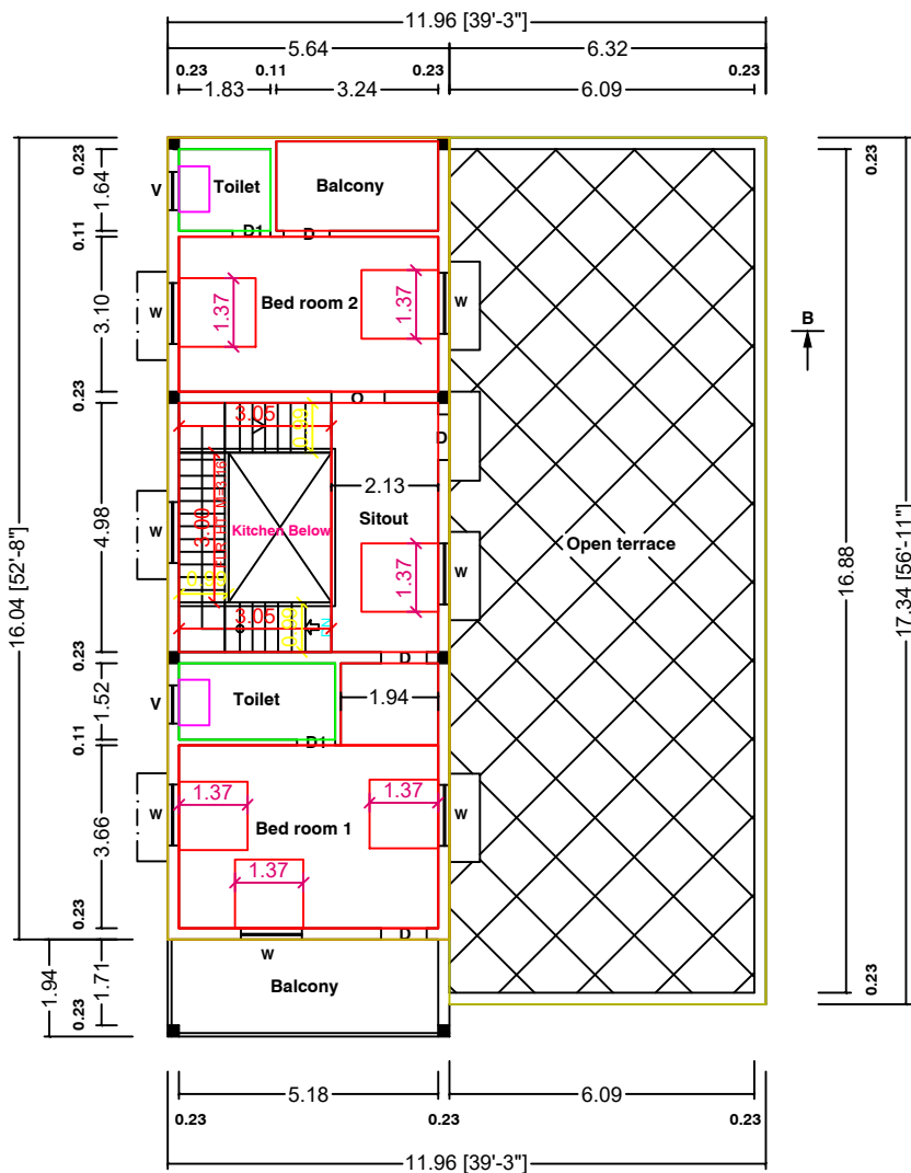
FLOOR-1 (FIRST) PLAN (FACING SOUTH)
