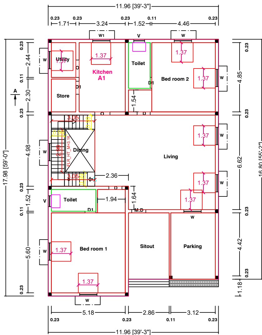
FLOOR-0 (GROUND) PLAN (FACING SOUTH)
