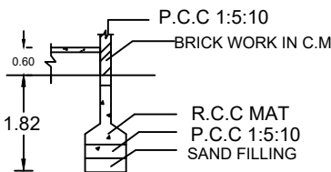
FOUNDATION DETAILS
