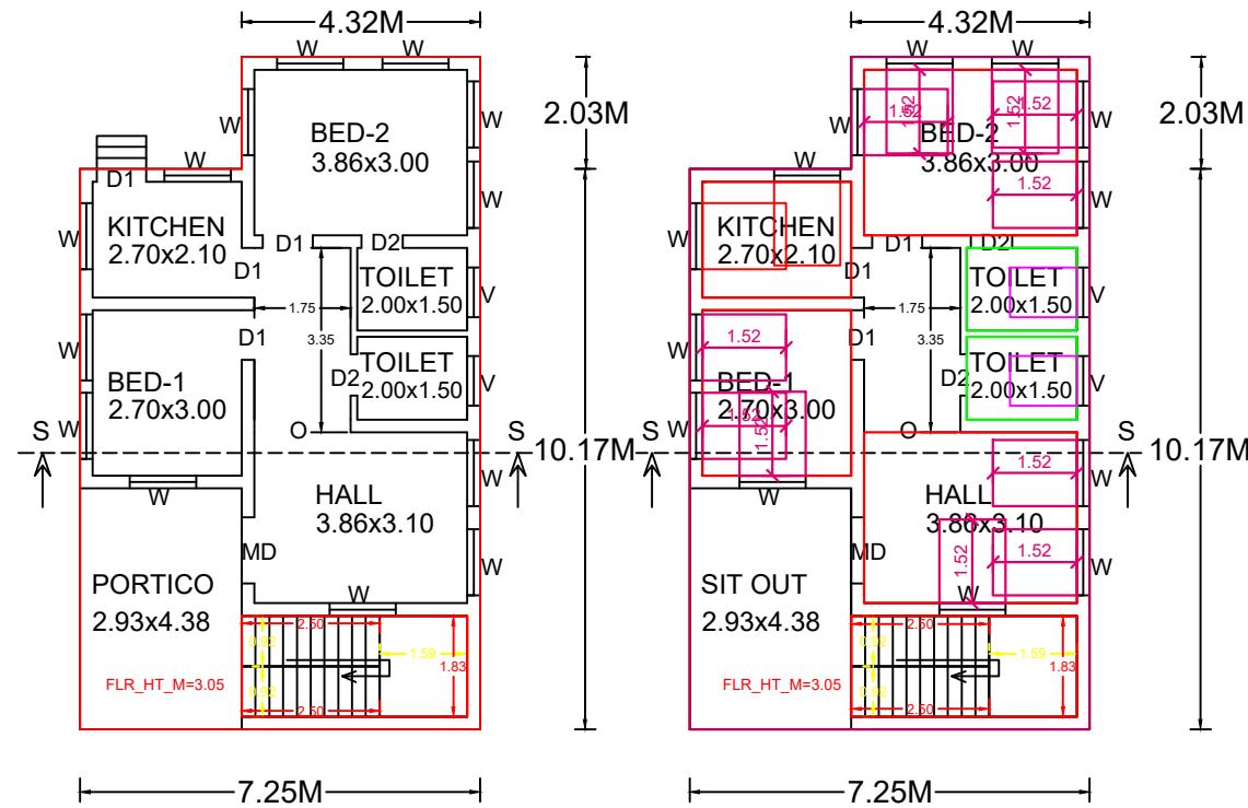
GROUND FLOOR
