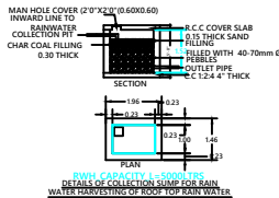
DETAILS OF COLLECTION TANK FOR RAIN WATER
