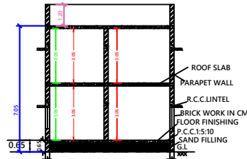
SECTION ON SS
