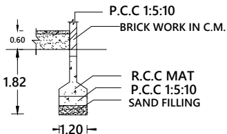
FOUNDATION DETAILS
