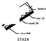
STAIR
