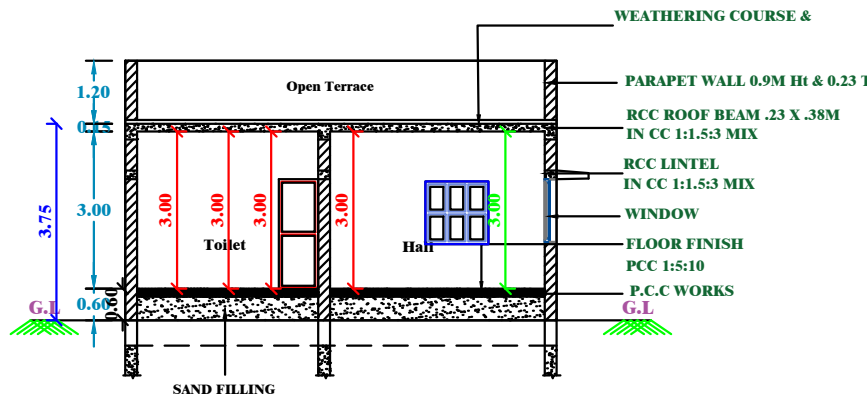
SECTION-XX
