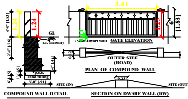
COMPOUND WALL DETAIL
