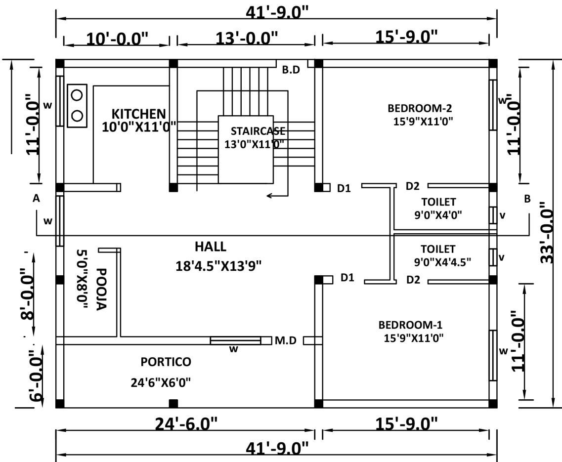
GROUND FLOOR PLAN (G.F)
