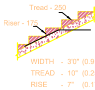
STAIR-CASE DETAILS (NOT TO SCALE)
