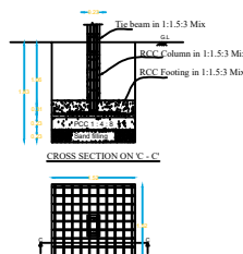
COLUMN FOUNDATION DETAILS
