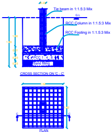
COLOUMN FOUNDATION DETAILS
