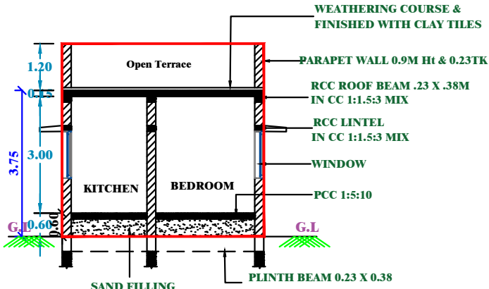
SECTION-XX
