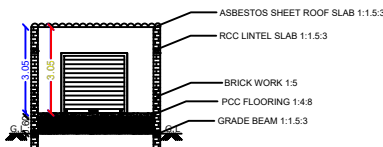
SECTION ON AB
