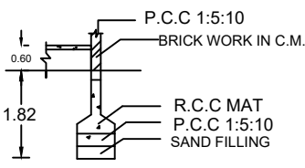
FOUNDATION DETAILS
