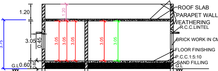
SECTION ON SS
