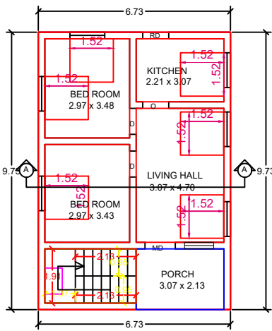
PRO.GOUND FLOOR PLAN
