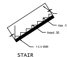
STAIR
