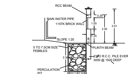
RAINWATER HARVESTING
