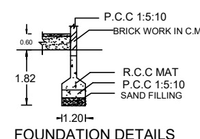
FOUNDATION DETAILS
