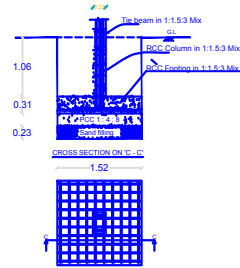
COLOUMN FOUNDATION DETAILS
