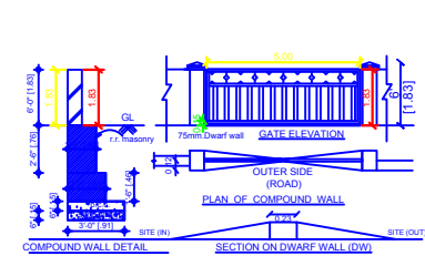
COMPOUND WALL DETAILS
