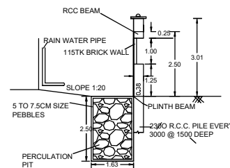
RAINWATER HARVESTING
