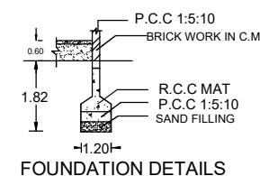
FOUNDATION DETAILS
