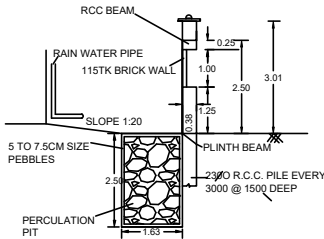
RAINWATER HARVESTING
