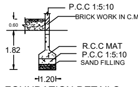
FOUNDATION DETAILS
