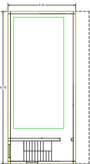
TERRACED FLOOR PLAN
