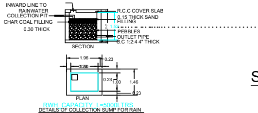
DETAILS OF COLLECTION SUMP FOR RAIN
