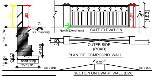
SECTION ON DWARF WALL (DW)
