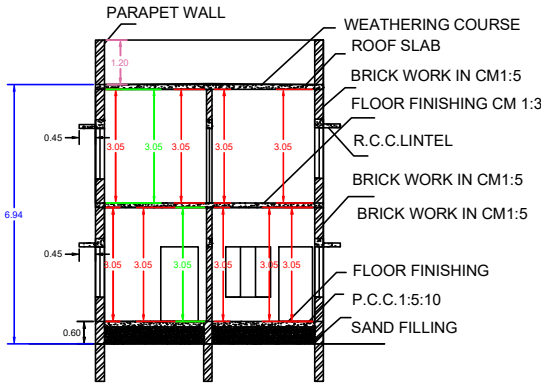
SECTION ON SS
