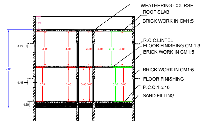
SECTION ON SS
