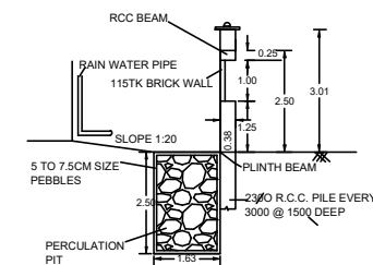
RAINWATER HARVESTING
