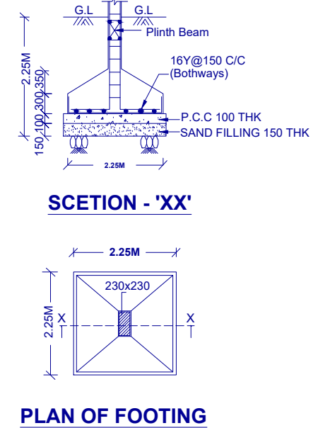
PLAN OF FOOTING
