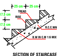
SECTION OF STAIRCASE
