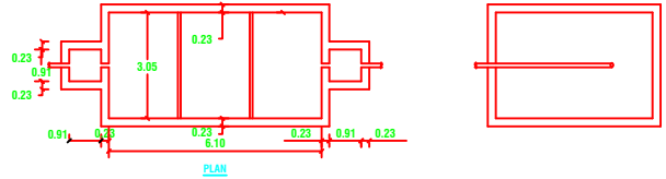
PLAN & SECTION OF SEPTIC TANK & DISPERSION TRENCH
