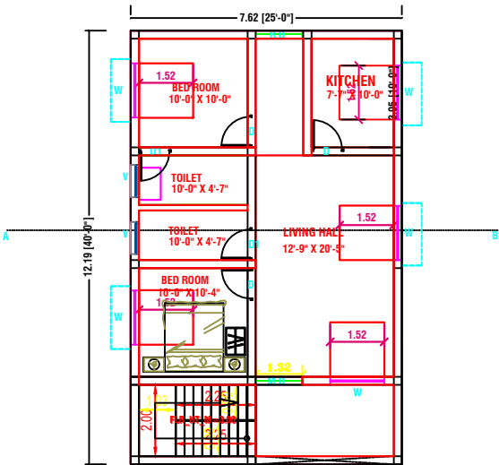
GROUND FLOOR PLAN (EAST FACING)
