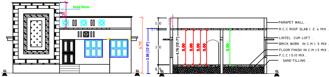
FRONT ELEVATION
