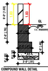
COMPOUND WALL DETAIL
