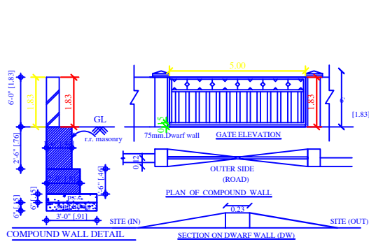
COMPOUND WALL DETAILS
