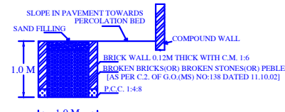
SECTION OF RAIN WATER PERCOLATION BED
