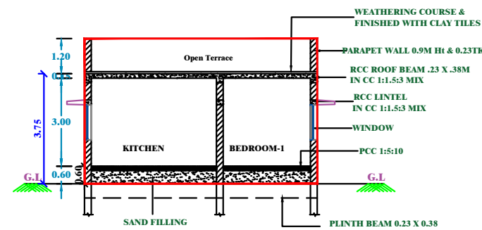
SECTION-XX
