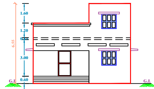
ELIVATION
