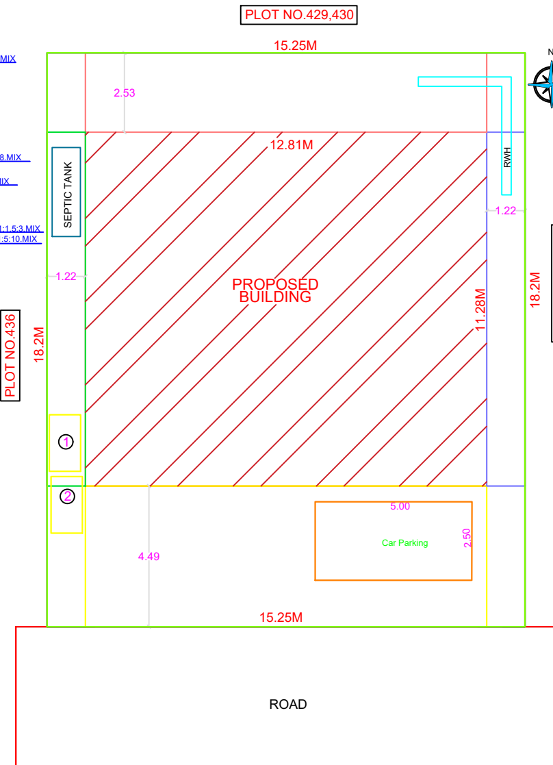
SITE PLAN
