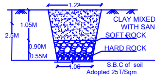
TRIAL PIT DETAIL
