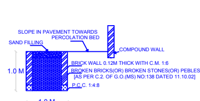
SECTION OF RAIN WATER PERCOLATION BED
