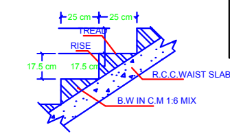
SECTION OF STAIRCASE
