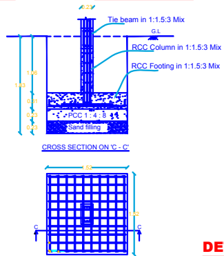
COLOUMN FOUNDATION DETAILS
